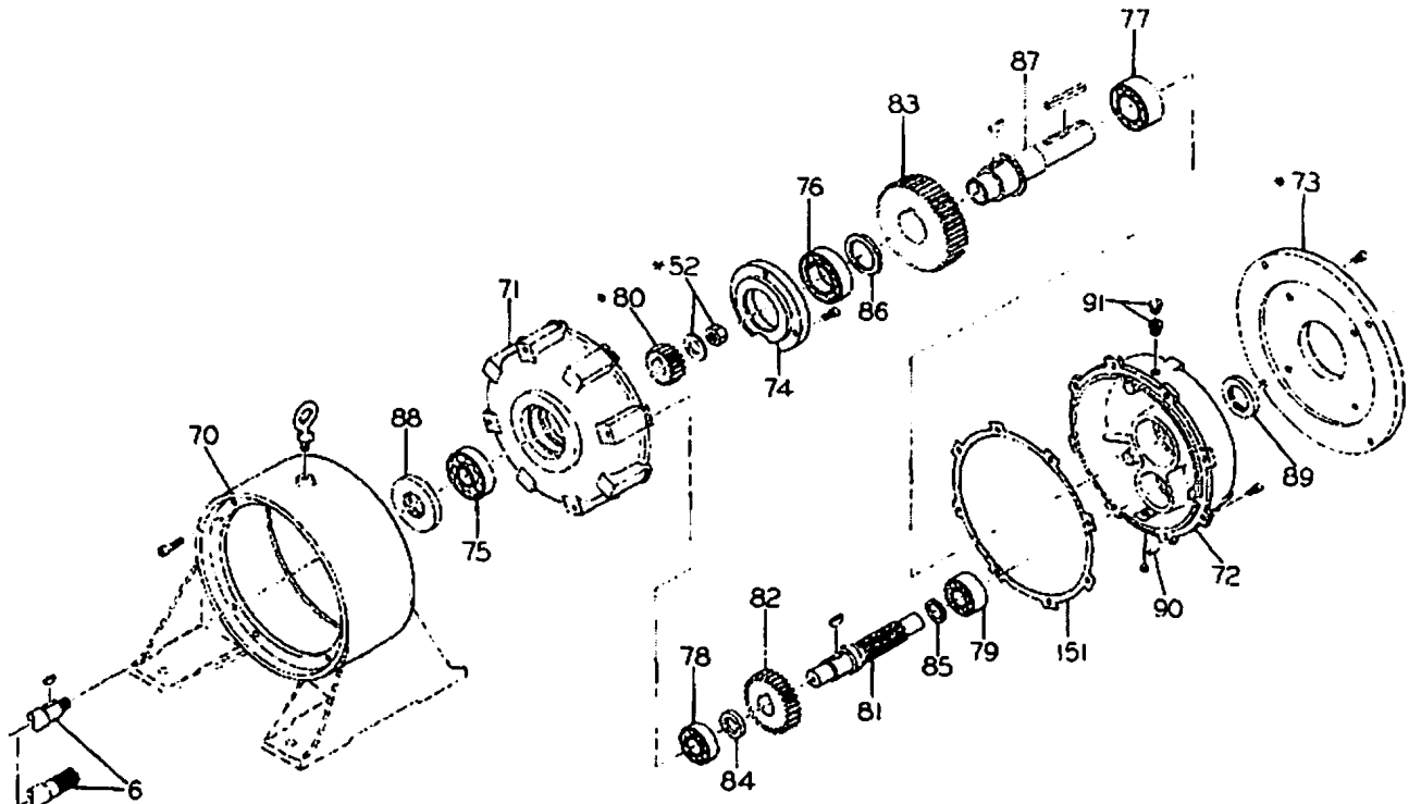
PARTS ILLUSTRATION DOUBLE REDUCTION HELICAL MOTOREDUCER TYPE S00D, S00E
